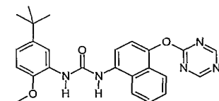
1-(5-tert-Butyl-2-methoxy-phenyl)-3-[4-([1,3,5]triazin-2-yloxy)-naphthalen-1-yl]-urea;
